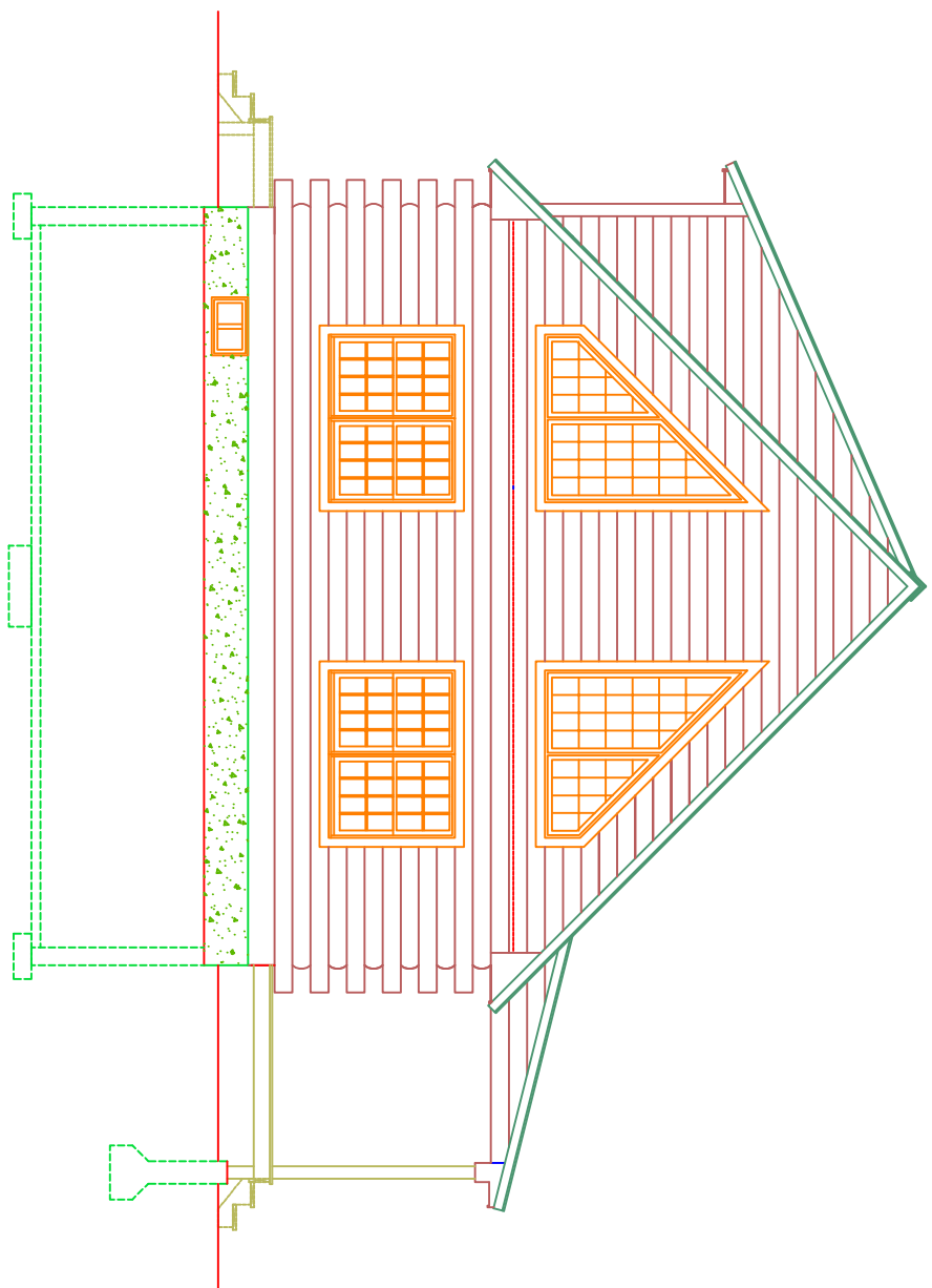
LEFT ELEVATION
